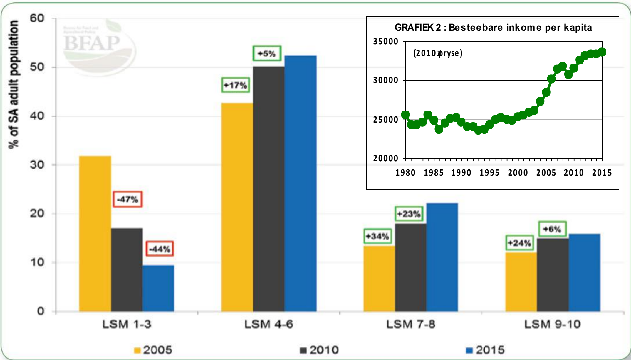
Figure 15: LSM class mobility: All adults for the period 2005, 2010 and 2015
